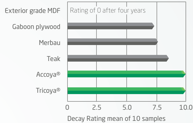
Four Year H3 Above Ground Testing. Borneo, Malaysia. ASTM Decay Rating.
