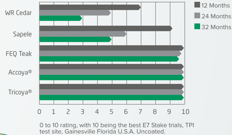
Decay Resistance
