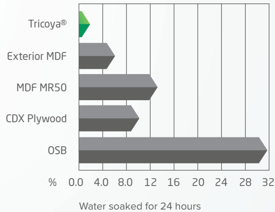
Thickness Swelling
